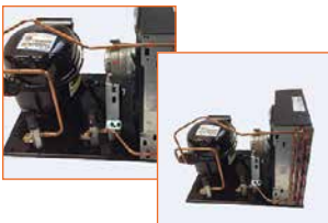
Condensing Unit 1/4 HP - 103CCON0003 1/3 HP - 103CCON0004 1/2 HP - 103CCON0002
